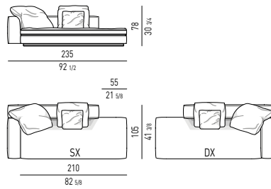
ELEMENTO TERMINALE PENISOLA CM 235 - SCHIENALE CM 180 OPEN-END ELEMENT WITH ARMREST CM 235 - BACKREST CM 180
