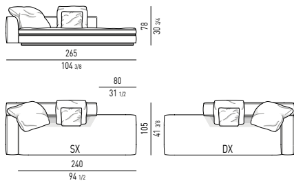
ELEMENTO TERMINALE PENISOLA CM 265 - SCHIENALE CM 185 OPEN-END ELEMENT WITH ARMREST CM 265 - BACKREST CM 185
