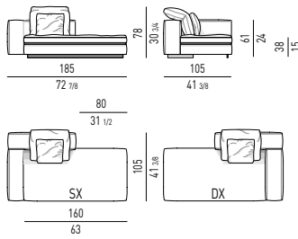
ELEMENTO TERMINALE PENISOLA CM 185 - SCHIENALE CM 105 OPEN-END ELEMENT WITH ARMREST CM 185 - BACKREST CM 105
